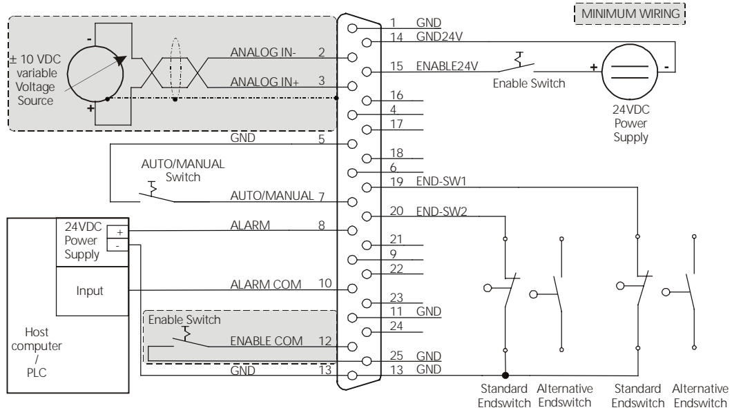
Figure 44: J3 Axis Signals Wiring, DSUB25 male cable to J3
