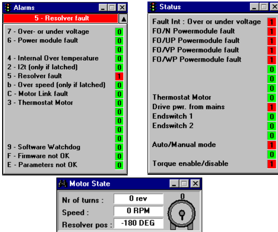
Figure 76: Drive GUI Indications
