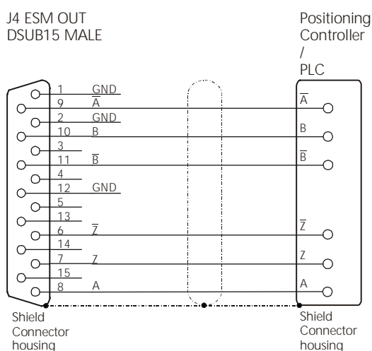
Figure 45: Encoder Output, DSUB15 male cable to J4
