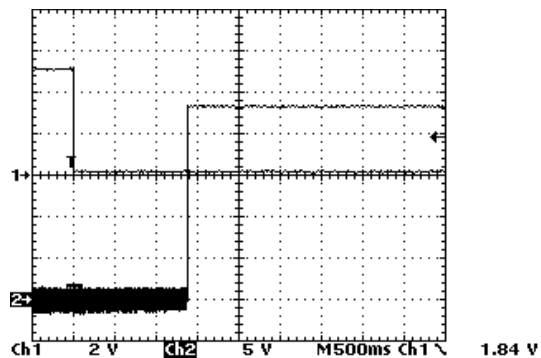
Channel 1: drive enable on pin J3:12 – 13 high(5VDC) = disable, low (0VDC) = enable Channel 2: monitoring relay
