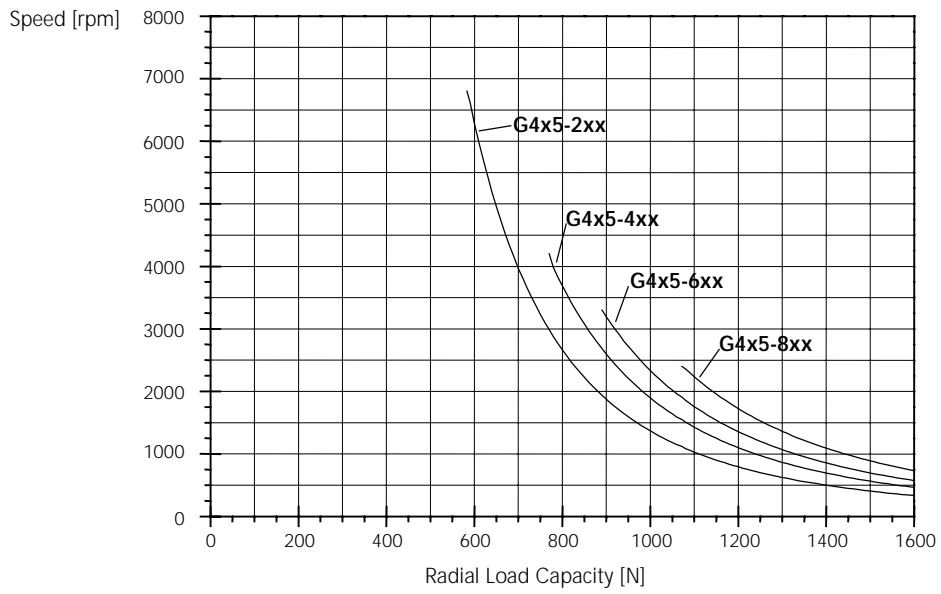
Figure 10: Radial Load Capacity G4x5
