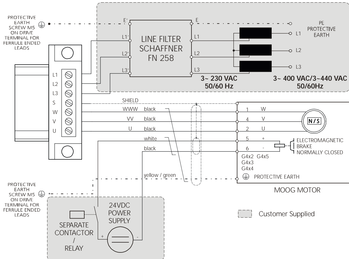
Figure 40: TBI Wiring
