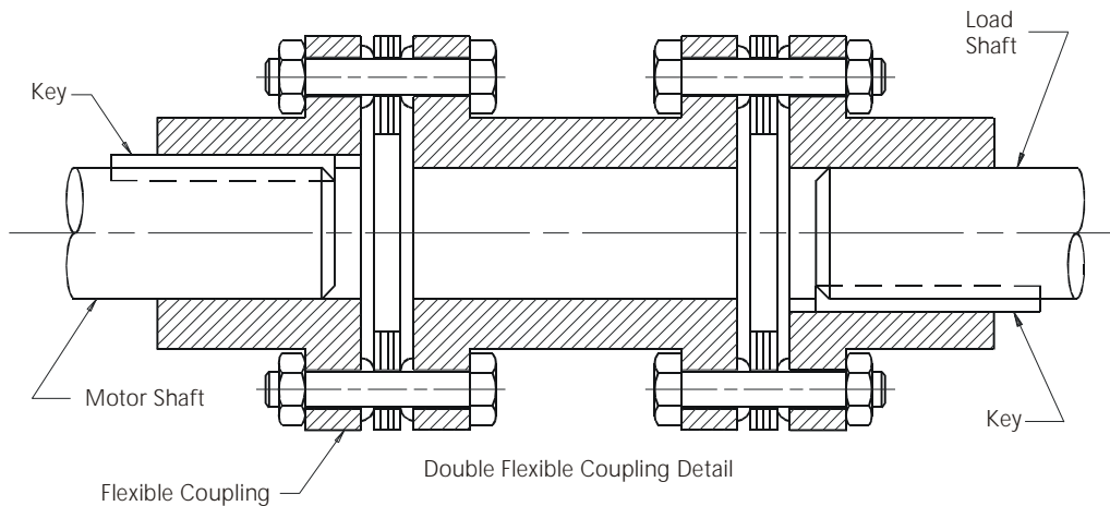
Figure 11: Motor Load Coupling
