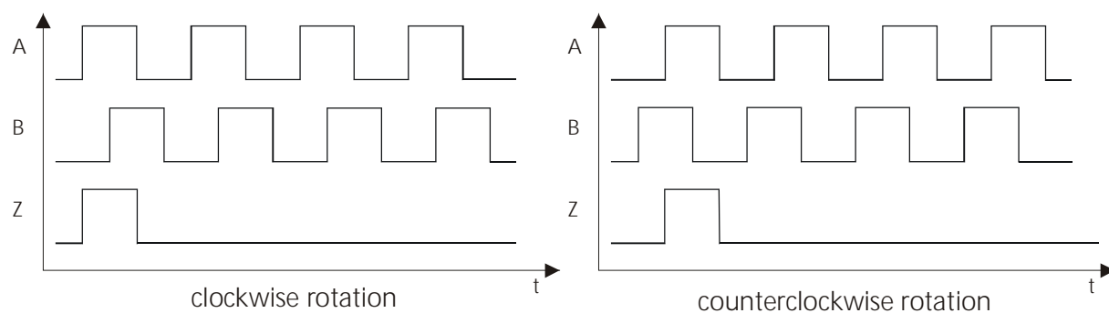
Figure 46: Definition of Encoder Signals, viewed from the shaft side
