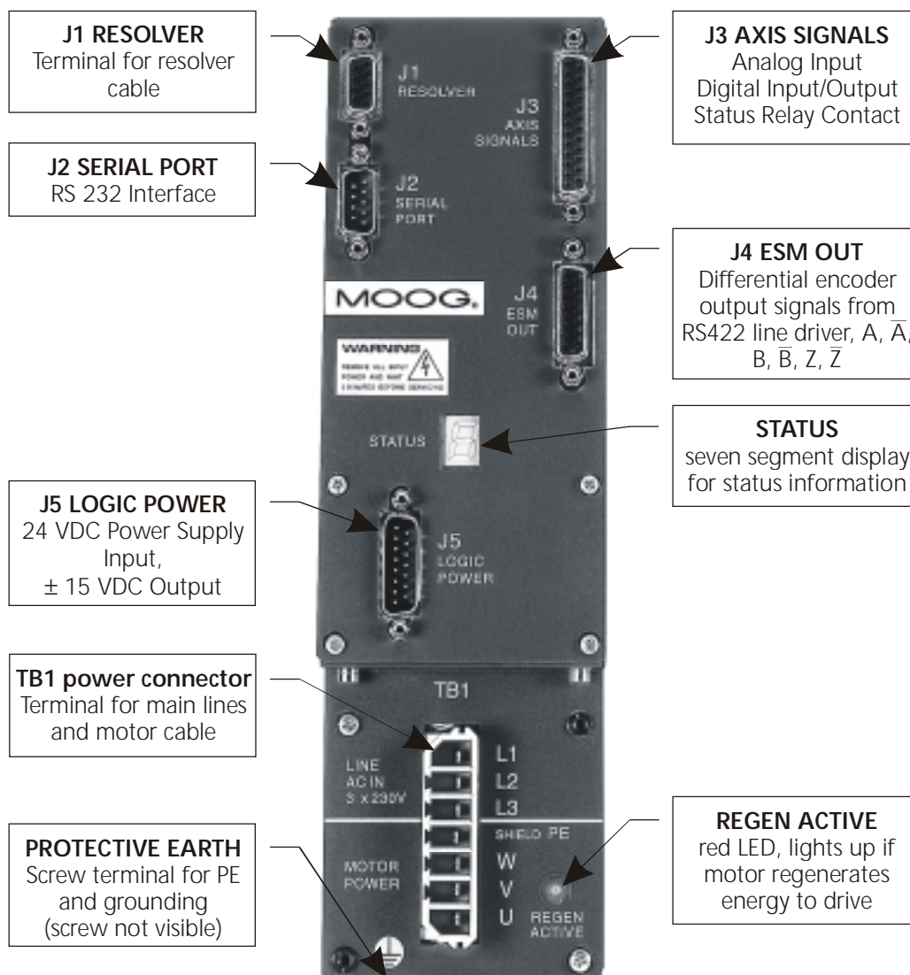
Figure 39: Wiring Overview
