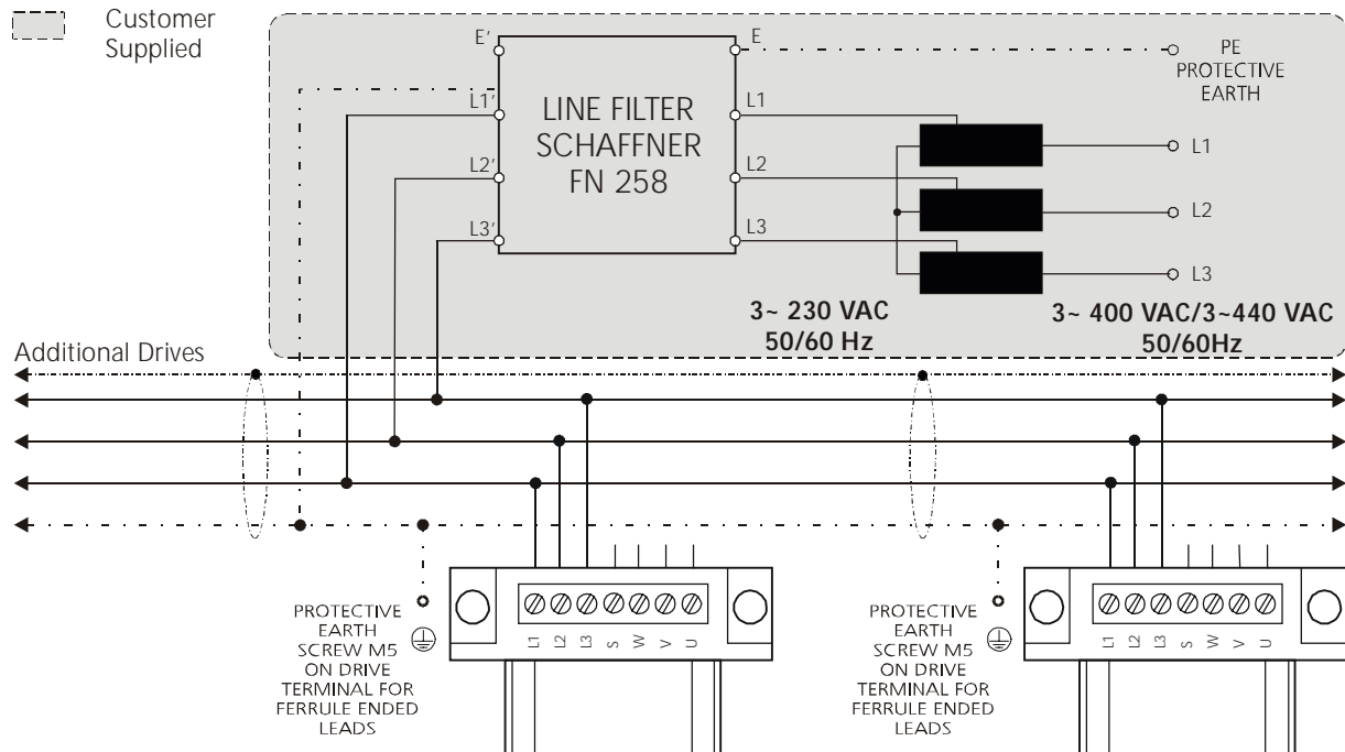
Figure 41: Multi Axis Wiring
