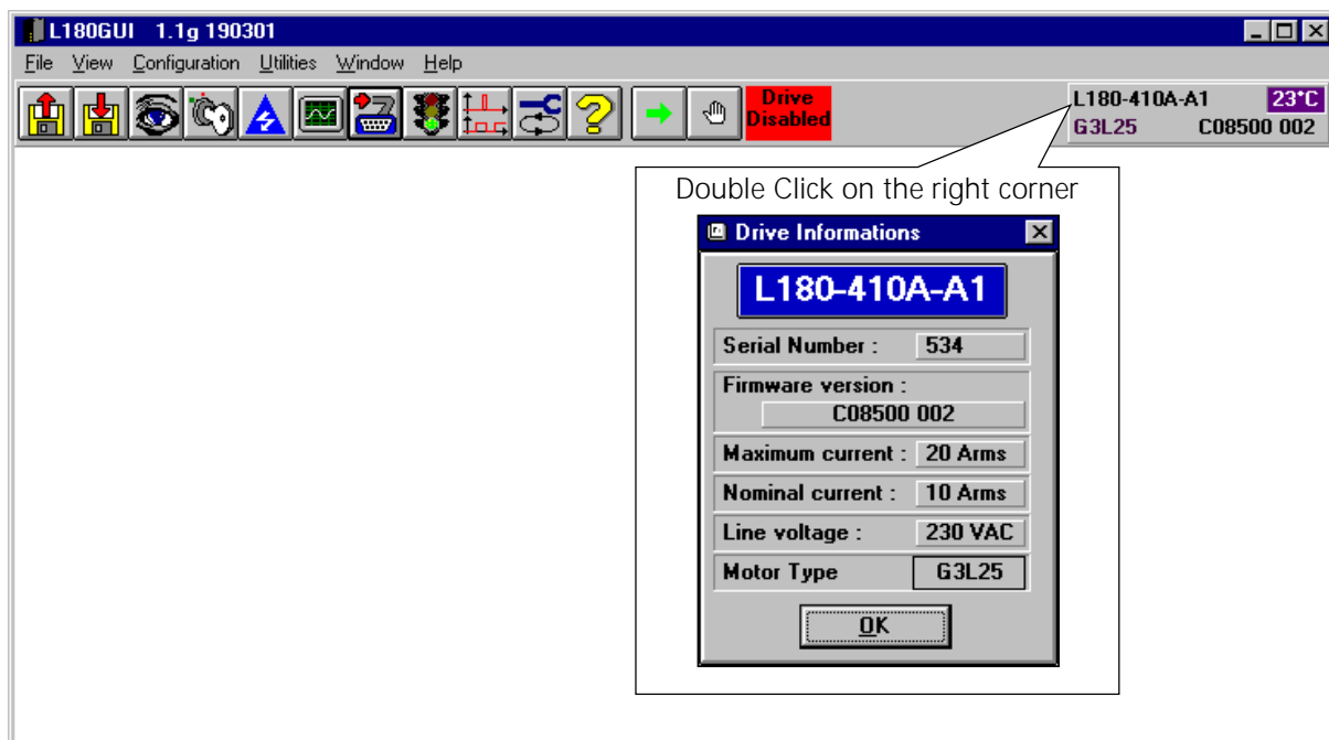
Figure 48: Main Window
