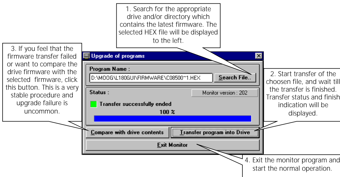
Figure 73: Firmware Upgrade
