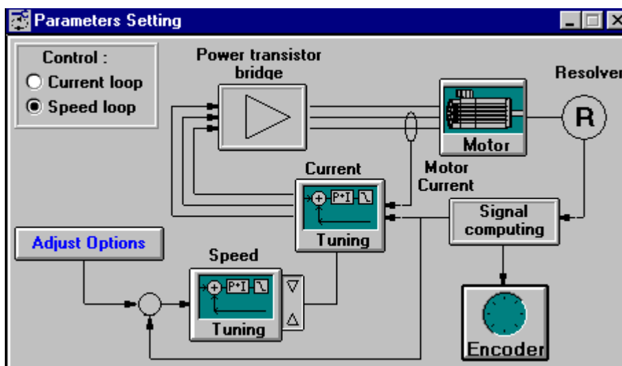
Figure 49: Parameters Setting
