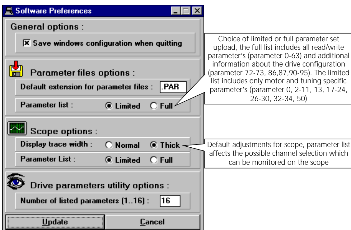
Figure 75: Preferences
