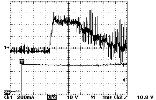
Channel 1: motor phase current Channel 2: monitoring relay
