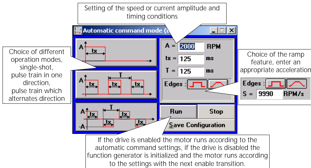
Figure 67: Automatic command mode
